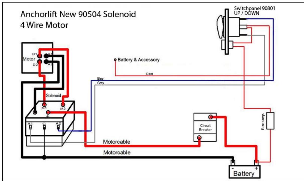
Wiring diagram for 4 wire motor Aquarius 2500 - 3000
