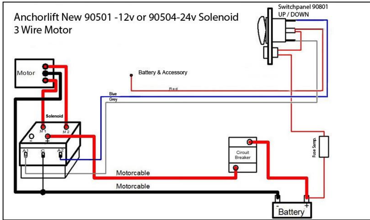
Wiring diagram for 3 wire motor Mako 1500 - 2000
